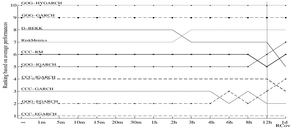
Figure 1: Consistency of the ranking based on average performance - Frobenius norm squared
