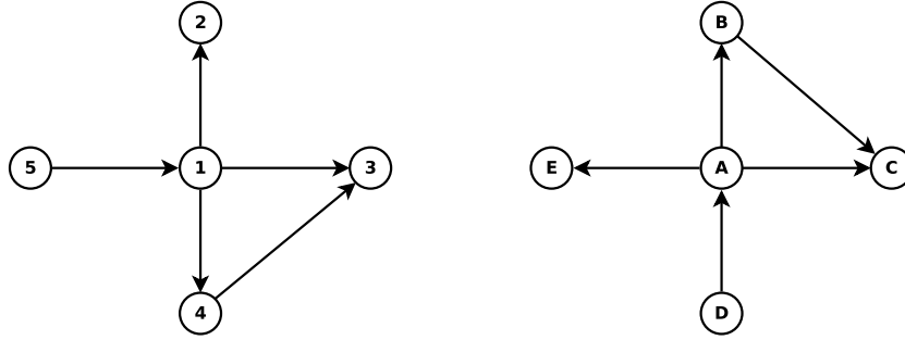
Figure 2.4: Example of graph isomorphism with f = \{(1, A), (2, E), (5, D), (4, B), (3, C)\} .
