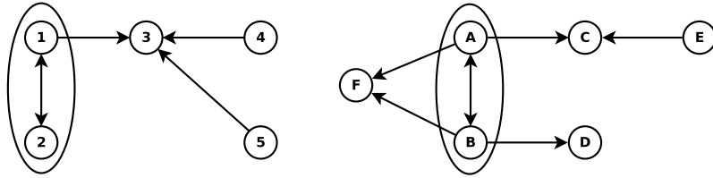
Figure 2.11: Instance where only the second pruning condition fails
