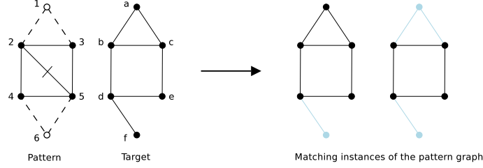
Figure 3.2: Example of approximate matching.
