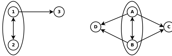
Figure 2.9: Instance where the subgraph is partial and not induced.
