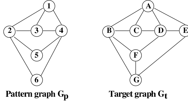
Figure 4.1: Instance of subgraph isomorphism problem.
