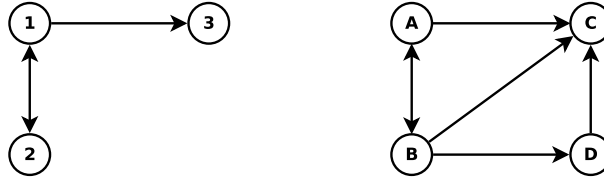
Figure 2.6: Example of partial subgraph isomorphism with f = \{(1, A), (2, B), (3, C)\} . There is no induced subgraph isomorphism, because the induced subgraph A, B, C has one more edge.
