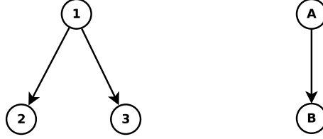
Figure 2.5: Example of graph epimorphism with f = \{(1, A), (2, B), (3, B)\} .
