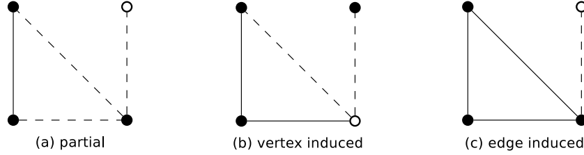
Figure 2.2: Example of partial, induced and edge-induced subgraphs.
