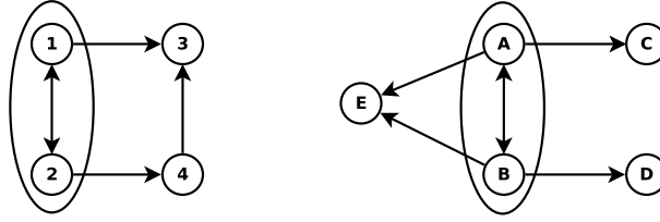
Figure 2.10: Instance where only the first pruning condition fails
