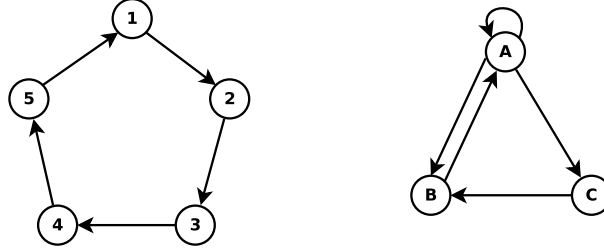
Figure 2.3: Example of graph homomorphism with f = \{(1, A), (2, B), (3, A), (4, B), (5, A)\} .
