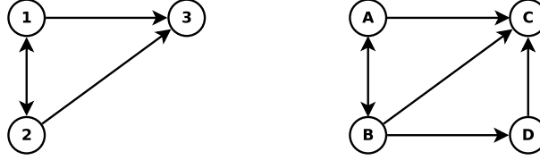
Figure 2.7: Example of induced subgraph isomorphism with f = \{(1, A), (2, B), (3, C)\} .
