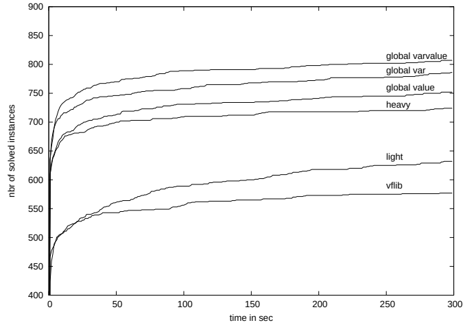
Figure 5.3: Results for global symmetries
