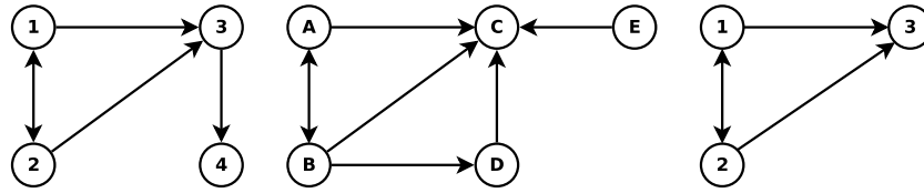
Figure 2.8: Example of maximum common induced subgraph with f = \{(1, A), (2, B), (3, C)\} . The resulting common subgraph is shown on the right.
