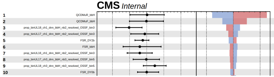
Figure 5.35. | The first ten leading nuisance parameters with the largest impacts on the fitted signal strength \hat{\mu} assuming no signal ( \hat{\mu}=0 ) ranked from highest impact to lowest. The fitted DNN templates corresponding to full run2 data, nb2 + nb3 - resolved category, (ee + \mu\mu + \mu e) combined lepton flavours, and for bbH signal mass parameters (m_H, m_A) = (379, 44.72) GeV. The left panel illustrate the shifts between post-/pre-fit values ( \hat{\Theta} - \Theta_0 ) and uncertainties of these parameters, relative to their pre-fit uncertainty \Delta\Theta , while the right panel shows the impact of each parameter on the signal strength when varied \pm 1 standard deviation.
