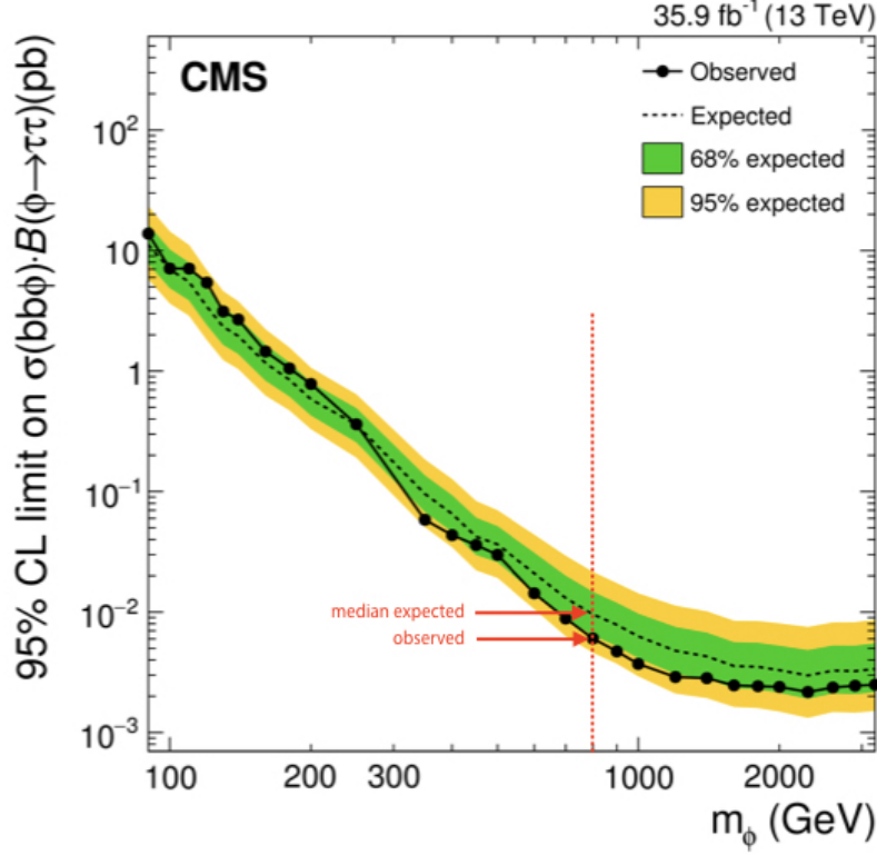
Figure 4.2. | The expected limit of \sigma \times B limits for the bb\phi \rightarrow \tau\tau process is shown under the background-only hypothesis, with \phi = (H \text{ or } A) in the context of the 2HDM. The median value under this hypothesis, as well as the 68% and 95% intervals of \mu \pm 1 and \mu \pm 2 \sigma bands respectively [111].
