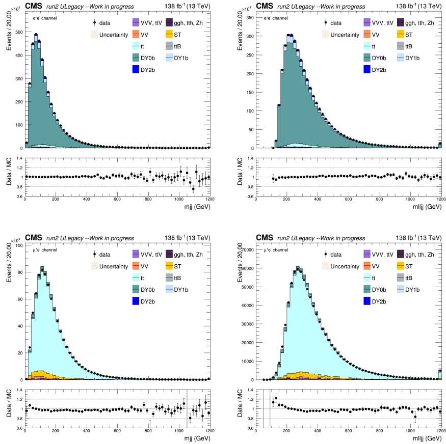
Figure 5.23. The m_{jj} (left), and m_{ljj} (right) invariant mass distributions are shown in the two lepton flavors ( ee (top) and \mu e (bottom)). The distributions are illustrated for ULegacy full run 2 data, simulated signal, and Monte-Carlo events after requiring two opposite charge same flavor leptons and at least two resolved AK4 jets. Error bars indicate statistical uncertainties.
