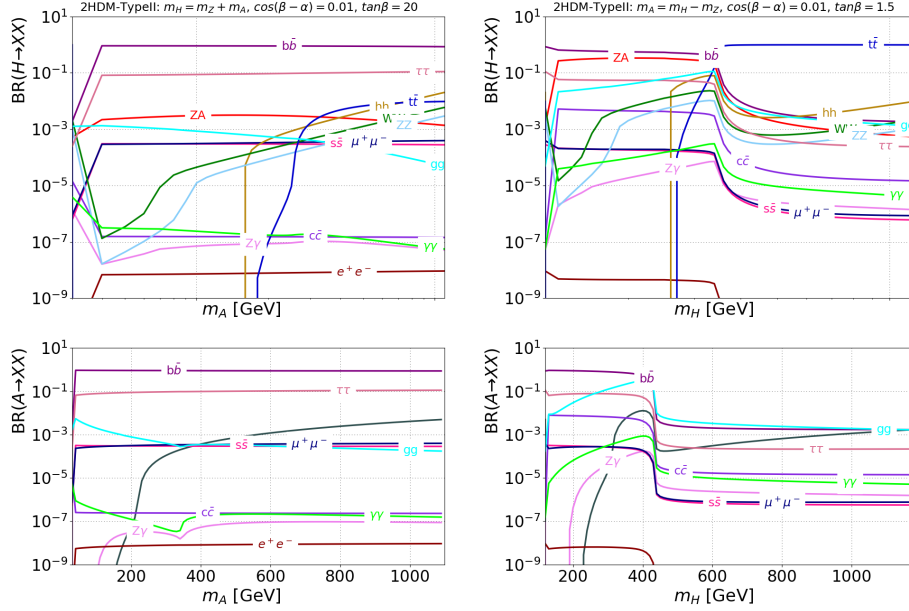
Figure 5.2. | H and A branching fractions as a function of m_A (left) and m_H (right) for the following set of parameters: \cos(\beta - \alpha) = 0.01 , \tan\beta = 20 (1.5) left (right). The plots are personal work and were created using the 2HDMC-1.8.0 tool [120].
