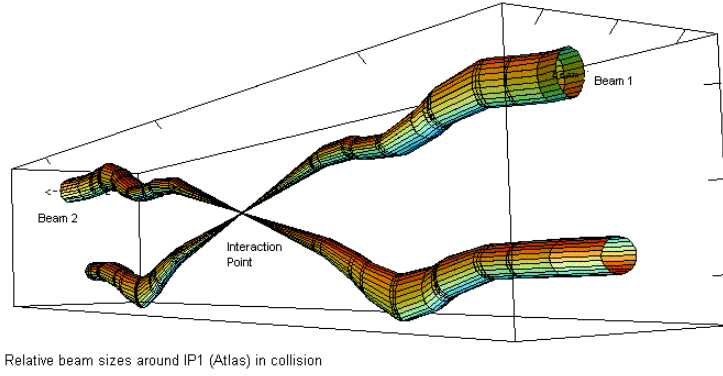
Figure 3.3. | Beam envelopes in the interaction region around point 1 ATLAS showing how the beam sizes are reduced on each side of the interaction point following the squeeze [80].
