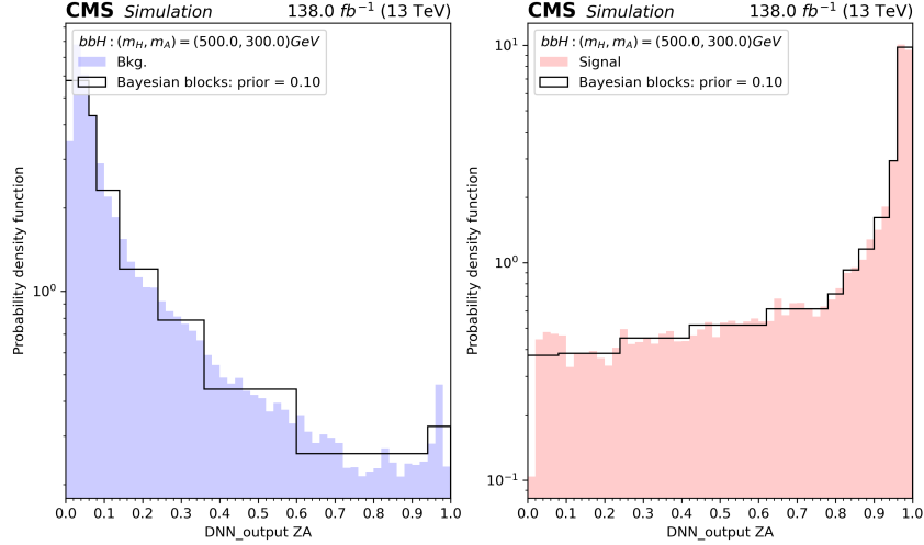
Figure 5.31. The Bayesian blocks binning is shown in black using “background-only” (left), “signal-only” (right) DNN scores template for signal mass hypothesis consisting of m_H = 500 GeV and m_A = 300 GeV. Events are constructed in nb = 2 -resolved category, ee + \mu\mu channel. The Bayesian blocks are defined from a uniform DNN template of 50 bins shown in (red) and (blue) for signal and background events respectively.
