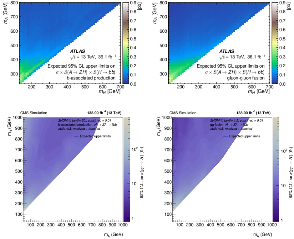
Figure 5.45. Upper bounds at 95% CL on the production cross-section times the branching ratio B(A \rightarrow ZH) \times B(H \rightarrow b\bar{b}) in pb (ATLAS) and on the cross-section in fb (CMS). These limits are determined separately for b-associated production (left) and gluon-gluon fusion (right). The top plots display the expected upper limits for ATLAS results [155], while our own results are presented at the bottom. An updated version of our results can be found in [153].
