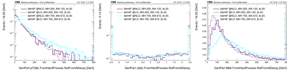
Figure 2.2. | Transverse momentum (left), pseudo-rapidity (middle), and the invariant mass (right) of the two hardest B hadrons at both LO+PS (dashed line) and NLO+PS (solid line).
