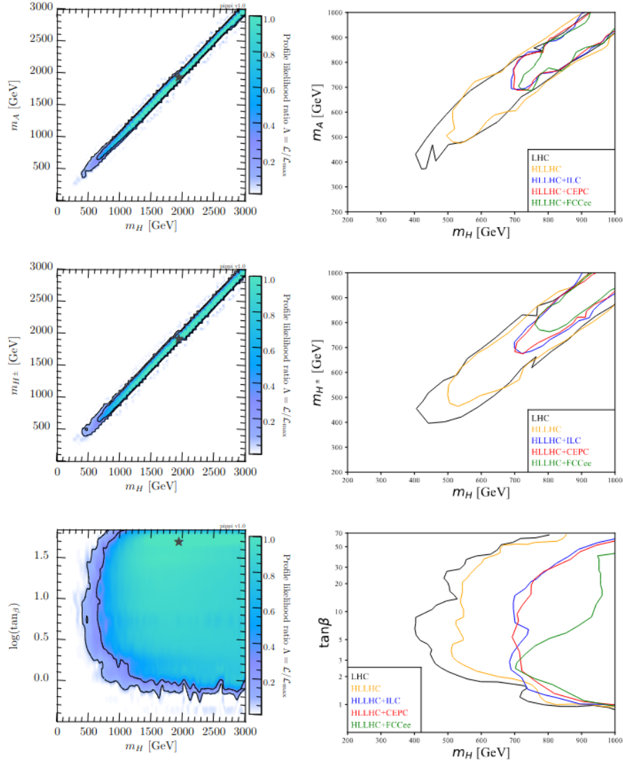
Figure 6.3. | Left panel: 1\sigma and 2\sigma global fit results in the m_A - m_H (top), m_H - m_H^\pm (middle), and m_H - \tan\beta (bottom), based on current measurements and theoretical constraints. Right panel: Comparison of current 2\sigma constraints (black) with future precision measurements from future colliders [158].
