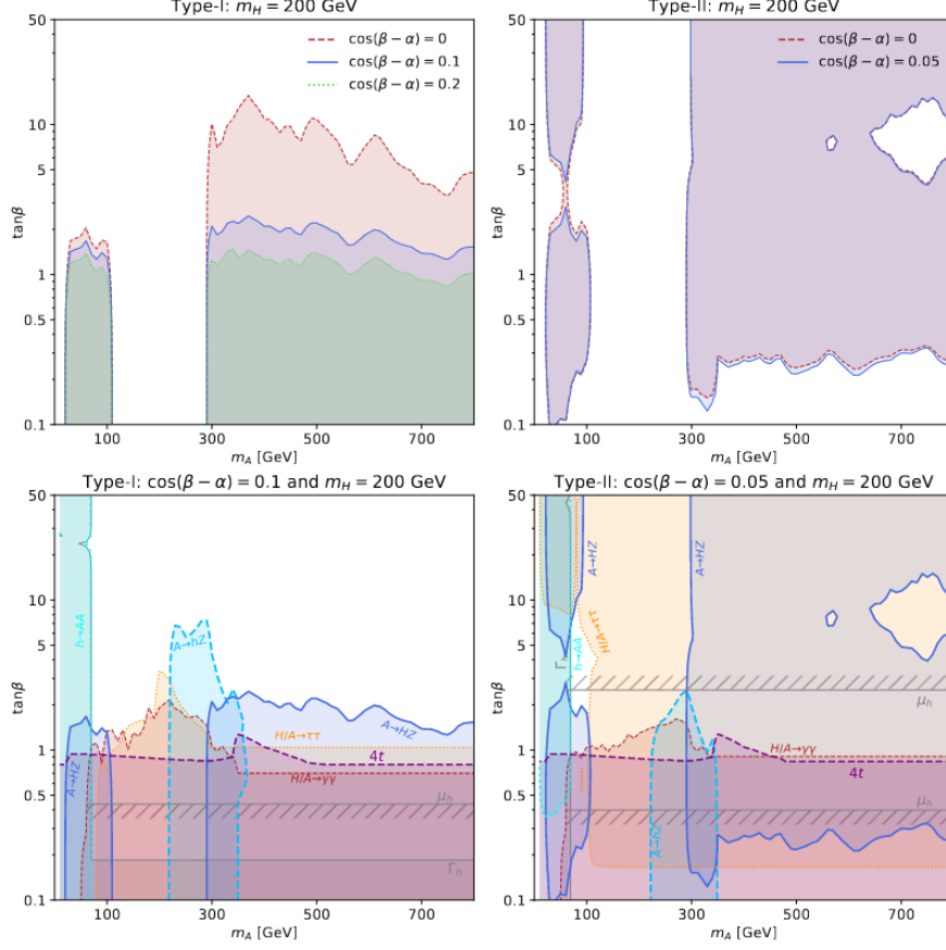
Figure 2.7. | Constraints of type-I (left) and type-II (right) 2HDM in \tan\beta vs m_A mass plane, assuming m_H = 200 GeV. Top: Parameter space excluded at 95% C.L. by the A/H \rightarrow ZH/ZA search for \cos(\beta - \alpha) = 0 (red), 0.1 (blue) and 0.2 (green) in the left panel and \cos(\beta - \alpha) = 0 (red) and 0.05 (blue) in the right panel. Bottom: Constraints at 95% C.L. for \cos(\beta - \alpha) = 0.1 from LHC searches for A \rightarrow ZH (blue), A \rightarrow Zh (dashed dark blue), H \rightarrow AA (dashed cyan), H/A \rightarrow \tau\tau (dotted orange), H/A \rightarrow \gamma\gamma (dashed brown) and 4t production (dashed magenta) as well as the global fit of SM-like Higgs couplings strength \mu_h (grey hatched region) and the Higgs width measurement \Gamma_h (grey) [72].
