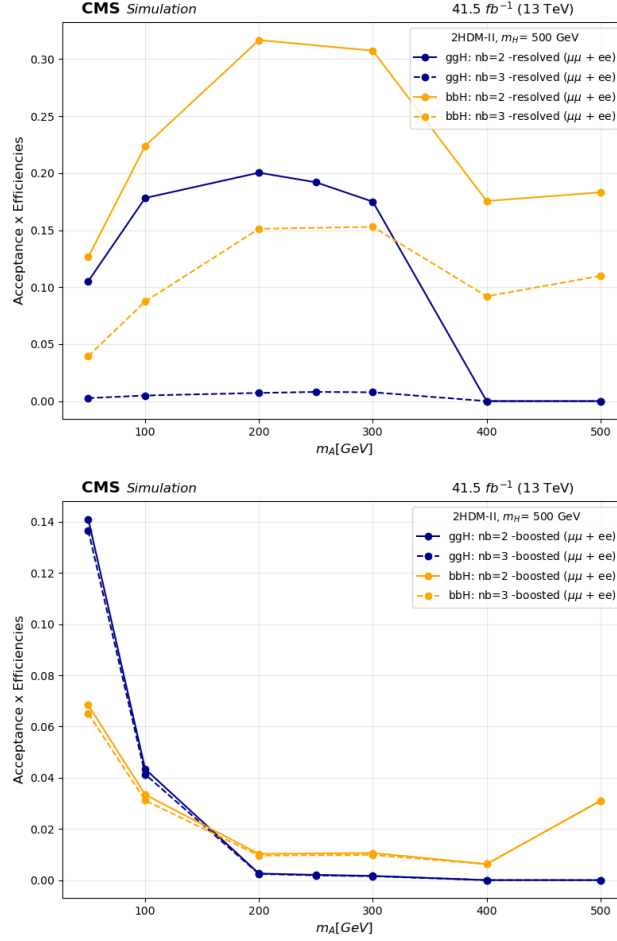
Figure 5.19. ggH and bbH signal acceptance times efficiency as function of m_A for a Heavy Higgs bosons H mass m_H = 500 GeV. The results are shown for the events passing the signal region selections nb=2 and nb=3 in the resolved (top) category, similarly boosted (bottom).
