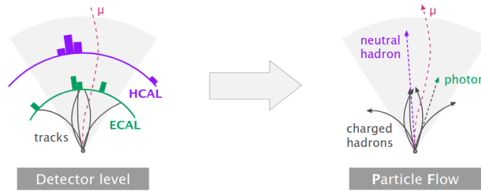
Figure 3.25. | Schematic view of the Particle-Flow PF concept: a combination of signals from different sub-detectors to construct objects, and represent individual particles with defined types [89].
