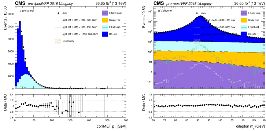
Figure 5.17. | 2016 ULegacy pre-/post-VFP corrected p_T^{\text{miss}} for xy-\phi modulation (left) and m_{ll} (right) in the nb=2 -resolved ( \mu\mu ) category.
