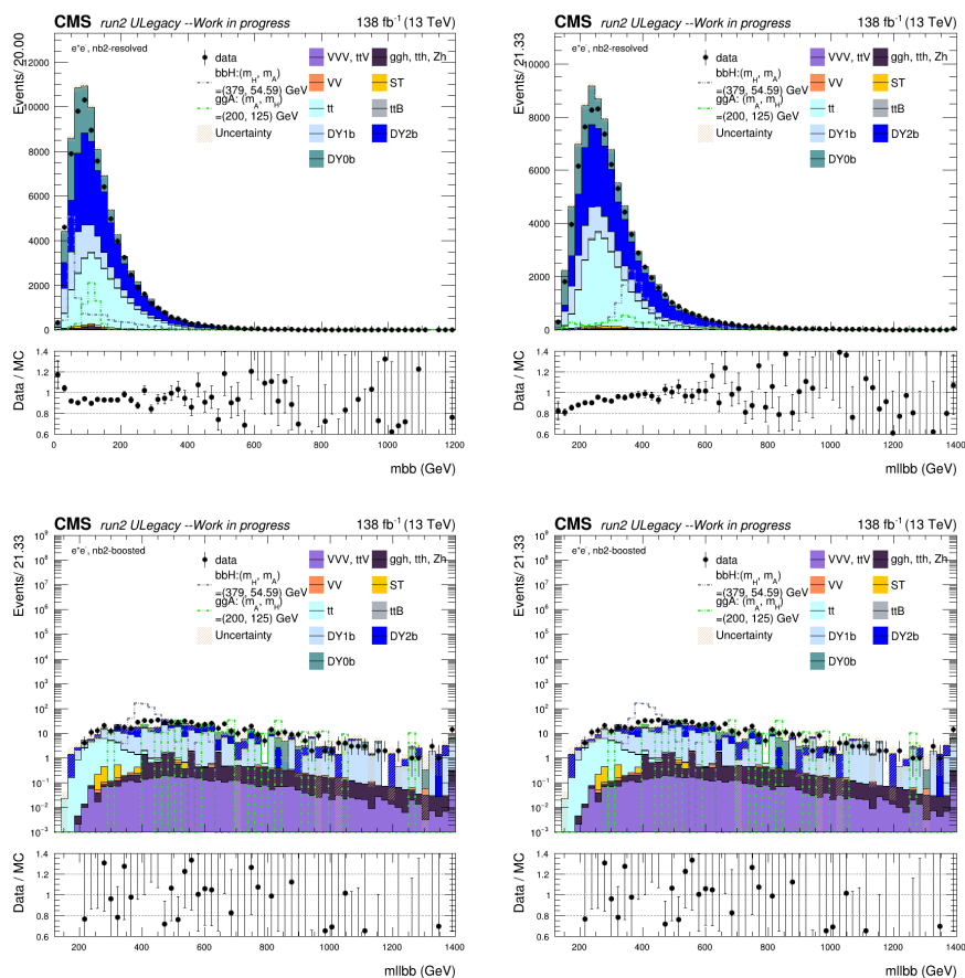
Figure 5.24. The m_{bb} (left), and m_{lbb} (right) invariant mass distributions are shown in nb2 -resolved (top) and -boosted (bottom) category. The distributions are illustrated for ULegcay full run 2 data, simulated signal, and Monte-Carlo events. The signal scaled to the cross-section of the 2HDM excluding branching fractions. The event requirements are two opposite charge same flavor leptons ( ee ) and exactly two b-tagged AK4 jets that pass the DeepJet algorithm medium working point in the resolved category, while two subjet within the AK8 jet to pass DeepCSV tagger medium working point. Error bars indicate statistical uncertainties.
