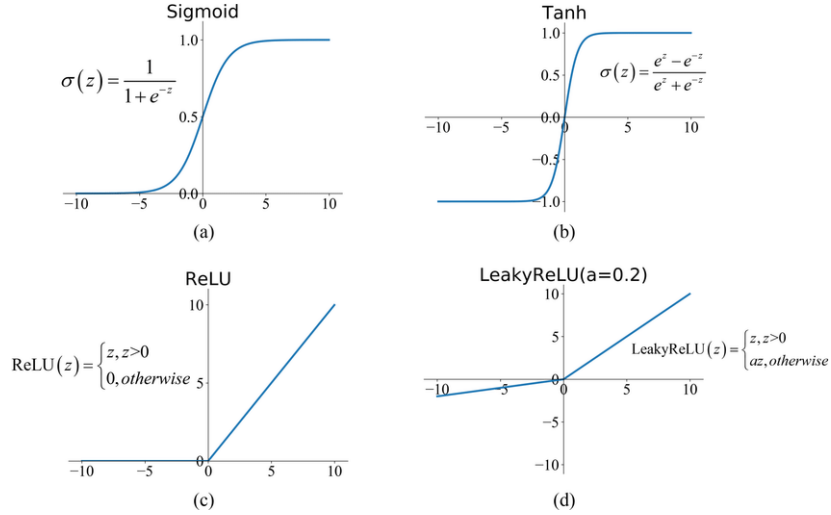
Figure 4.5. | Commonly used activation functions [114]: (a) Sigmoid, (b) Tanh, (c) ReLU, and (d) LReLU.
