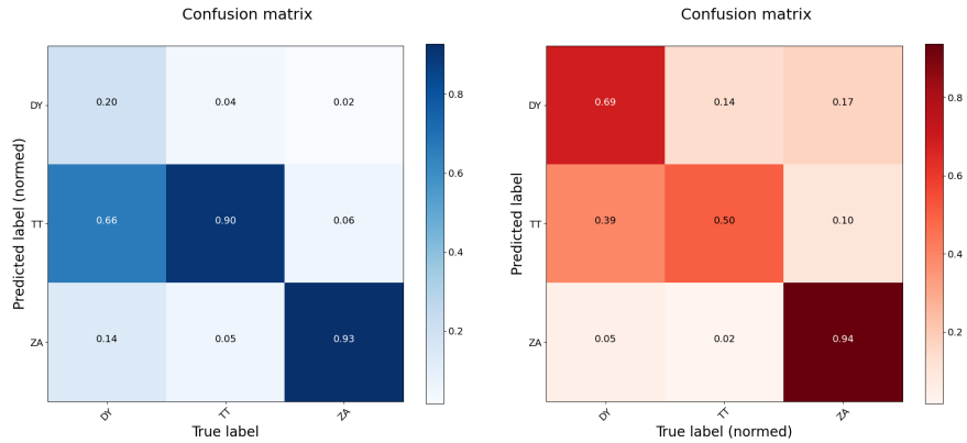
Figure 5.30. Confusion matrices show the network's multi-class classification performance. Both plots demonstrate for each true class their contributions to the different predicted labels. The values in these figures are normalized over the predicted conditions (left) and over the true conditions (right). Values on the diagonal represent the counting of the true prediction so the higher these values the better the predictive ability of the model.
