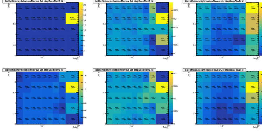
Figure 1.1. | 2016 Ulegacy postVFP b -tagging efficiencies for bbH resolved (top) and ggH resolved (bottom) derived for DeepJet tagger, medium b -tagging working point of b -jets (left), c -jets (middle) and light-jets (right).
