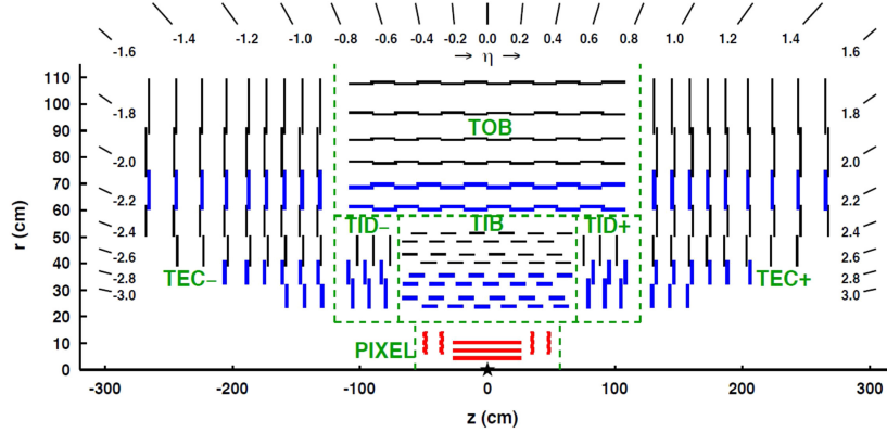
Figure 3.8. | A view of a tracker slice in the r-z plane. Pixel modules are shown in red, single-sided strip modules are depicted as black thin lines, and strip stereo modules are shown in blue thick lines [85].
