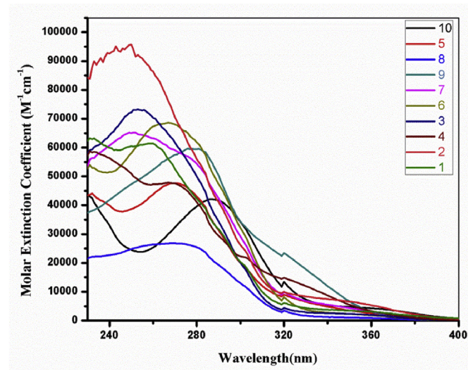
Fig. 6. Absorption spectra of functionalized pyridazine compounds ( 1–10 ).
