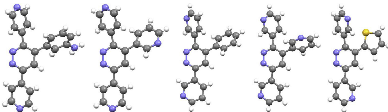
Fig. 3. Crystal structures of functionalized pyridazines 2 , 3 , 6 , 8 & 9 . Grey: C, Blue: N, White: H, Yellow: S.
