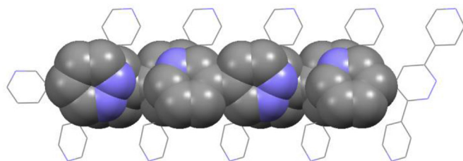
Fig. 5. Inter-molecular \pi - \pi stacked arrangement of pyridyl rings in crystal structure of 3 .
