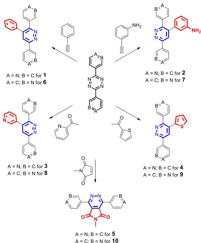
Scheme 1. One-step synthesis of pyridyl-functionalized pyridazines 1–10 .
