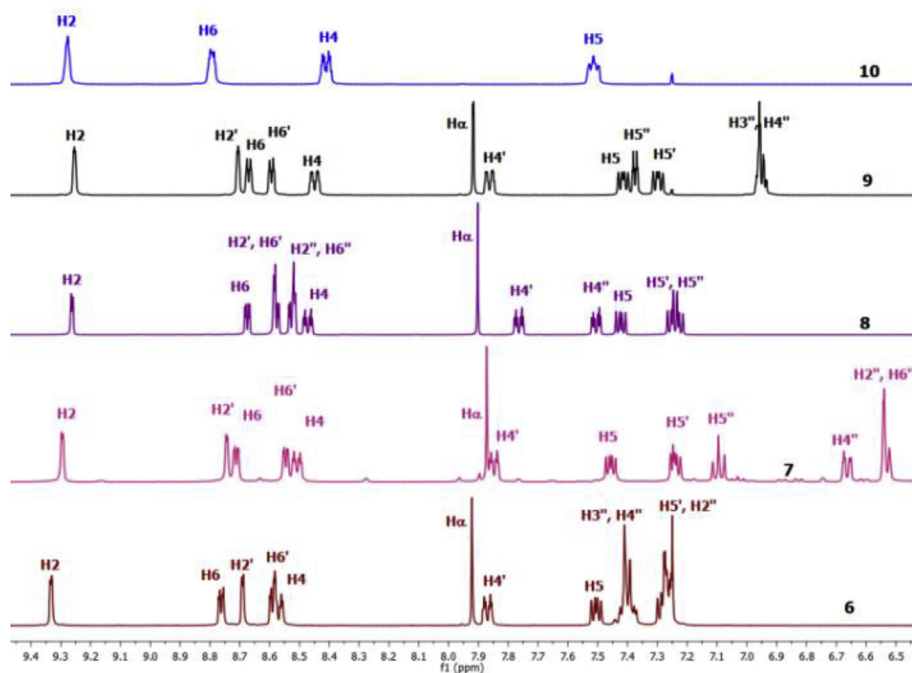
Fig. 2. ^1\text{H} NMR spectra of functionalized pyridazines 6–10 ( \text{CDCl}_3 , RT, 400 MHz).
