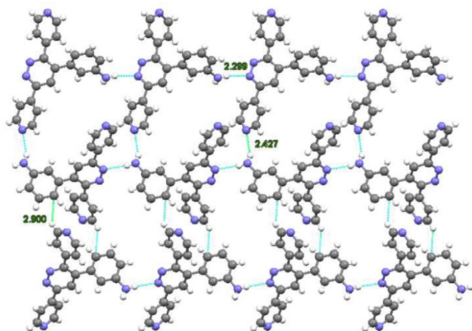
Fig. 4. Network of hydrogen-bonding and CH- \pi interaction formed molecules of 2 .
