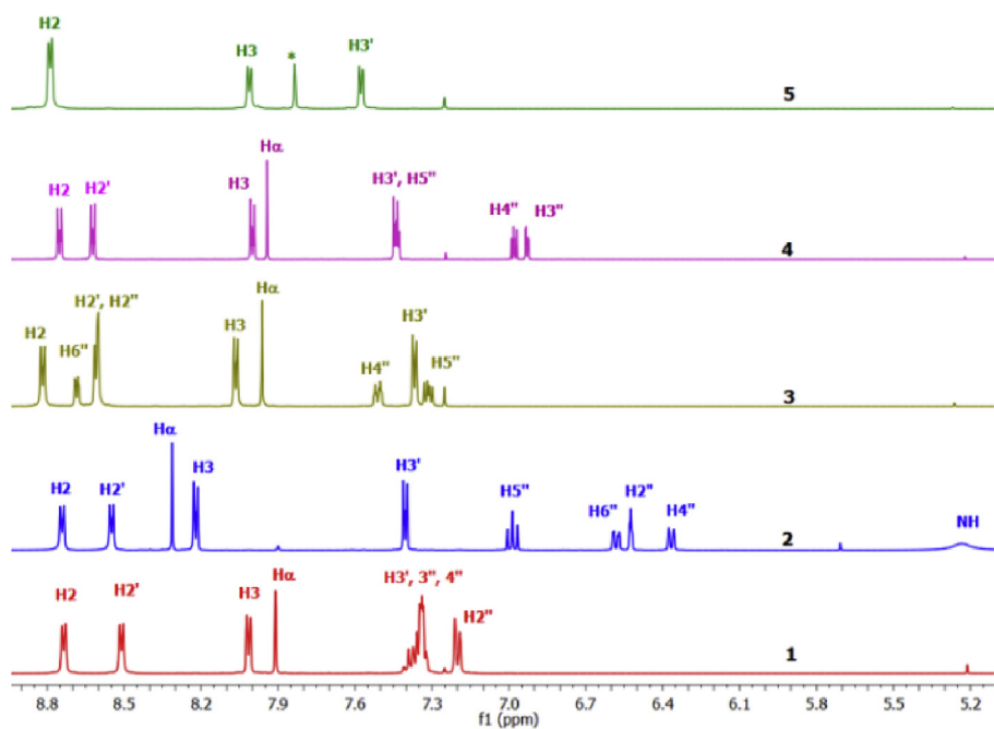
Fig. 1. ^1\text{H} NMR spectra of functionalized pyridazines 1–5 ( \text{CDCl}_3 , RT, 400 MHz).
