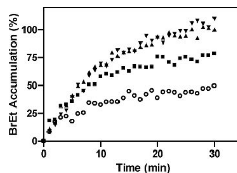
Figure 2. Accumulation of EtBr for 30 min in the presence and absence of increasing reserpine concentrations ( \circ , 0 M; \blacksquare , 10 M; \blacktriangle , 30 M; \blacktriangledown , 50 M). Experiments were performed in triplicate.
