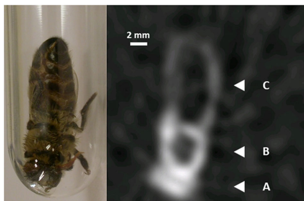
Fig. 3 2D EPR image of the honey bee. The data acquisitions are from the EPR peak recorded at room temperature at g = 2.004\text{--}2.005 . Note that the signal is almost exclusively contained in the periphery of the insect. A: Head. B: Thorax. C: Abdomen
