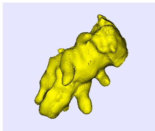
Fig. 4 Volume-rendered image of the presence of free radicals (3D image). The data acquisitions are from the EPR peak recorded at room temperature at g = 2.004\text{--}2.005 . Note the clear delineation of the abdomen, the thorax, the legs, the head, and the proboscis
