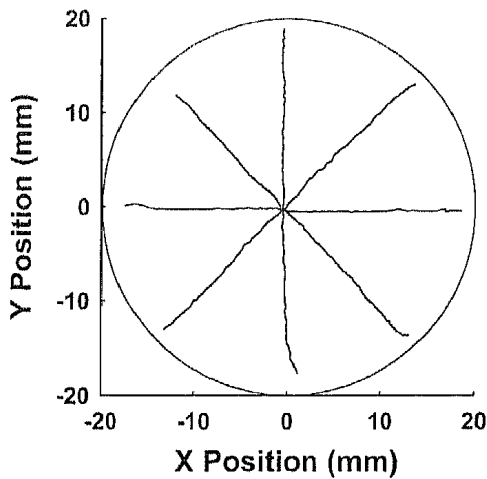
Figure 3. Reconstructed centre of pressure of a contacting force applied along four 45° spaced diameters on the transducer's plate (circle).
