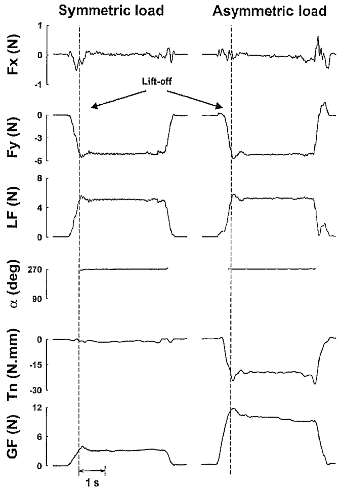
Figure 2. Typical traces of one grip lift trial in the symmetric (left panel) and asymmetric (right panel) load conditions (mass = 510 g). Presented over time are the horizontal ( F_x ) and vertical ( F_y ) components of the load force, the load force magnitude (LF) and direction ( \alpha ), the normal torque ( T_n ) and the grip force (GF). The vertical dashed lines are aligned with lift-off. The direction of LF is not computed when LF = 0 N.
