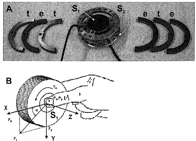
Figure 1. The instrumented device. (A) Fragmented view with three tungsten carbide (t) and three Ertalon® (e) semi-rings. (B) The common coordinate system used to measure the load force (LF), the normal torque T_n around the Z-axis and the coordinates ( P_x , P_y ) of the centre of pressure.
