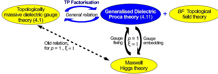
Figure 4.1: Duality relation between the physical sector of TMDGT (4.1) and the generalised first order formulation of dielectric Proca theories obtained through TP factorisation techniques. The dual Maxwell-Higgs model is recovered through a gauge embedding procedure in a very specific case. In blue: our contribution.
