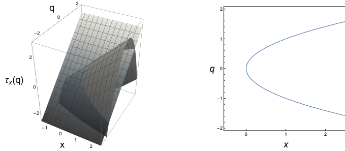
Figure 1.1: Graph of \tilde{\Delta} and \tau (left) and fixed point bundle of \tau (right).
