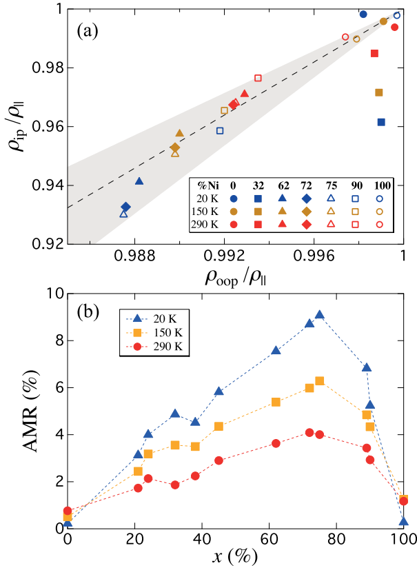
Fig. 3. (a) Comparison between the model (8) and the experimental variation of \bar{\rho}_{ip}/\rho_{||} versus \bar{\rho}_{oop}/\rho_{||} at H = 10 kOe for Ni_xCo_{1-x} interconnected fiber networks at the three temperatures of 20, 150, and 290K. The gray shaded area represents the calculated \bar{\rho}_{ip}/\rho_{||} in the angle range 40^\circ - 50^\circ . (b) Variation of the AMR ratio with respect to the Ni content at 20 K, 150 K, and 290 K [7].
