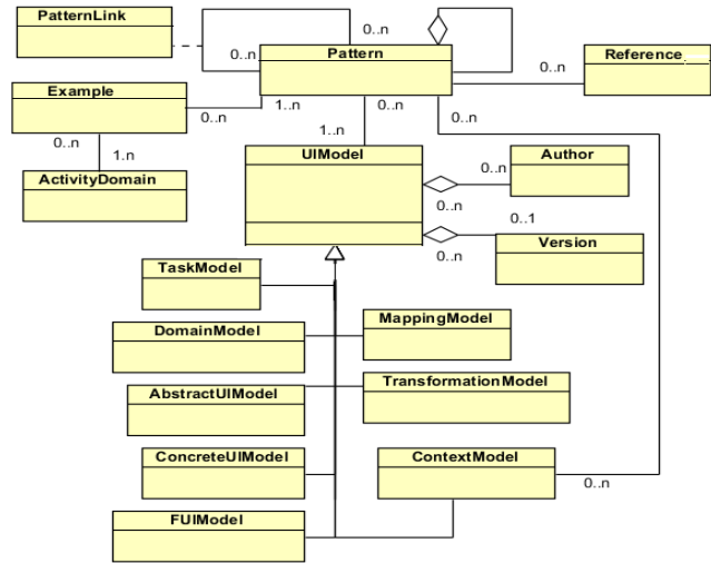
Figure 2: UI patterns extended from PLML represented in UML
