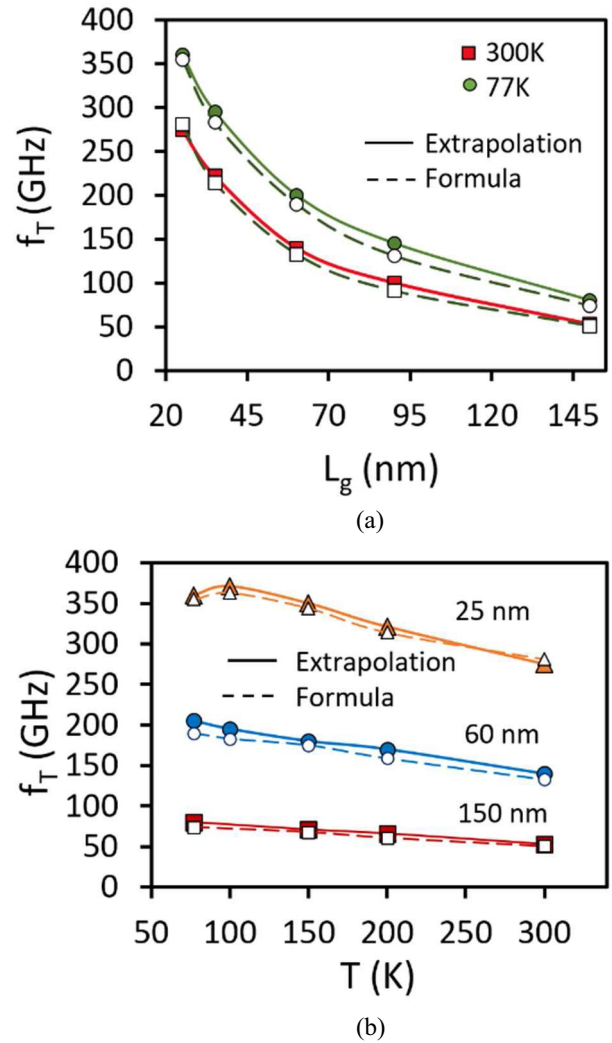
FIGURE 1. f_T vs. L_g for 77 K and 300 K (a) and vs. T for different L_g (b) by extrapolation (solid lines) and small-signal equivalent circuit extraction (dashed lines) in saturation for high V_{ds} ( V_{ds} = 1 V) and at V_{gs} that corresponds to maximum g_m .
