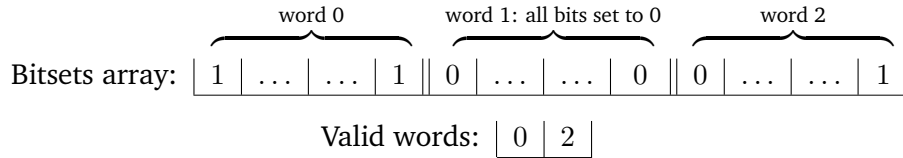
Figure 3.4: Sparse bitset
