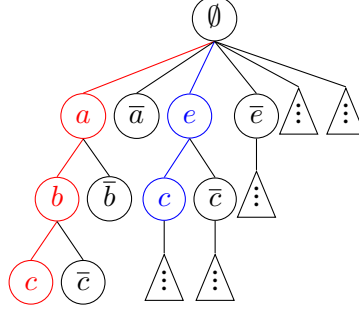
Figure 5.2: Search space
