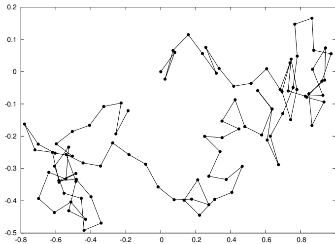
Fig. 1 A simulation of a particle released at (0,0) undergoing Brownian movement. Inspired by Perrin’s drawing of the Brownian motion of colloidal particles in water, viewed under the microscope (Figure 6 of Perrin, 1909, p. 81).
