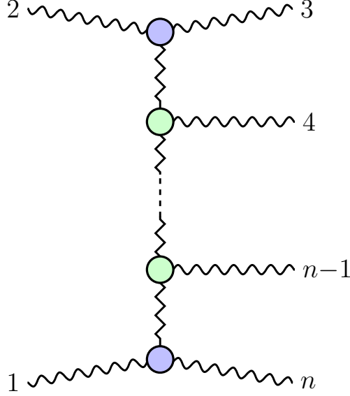
Figure 1: The factorized form of a tree-level amplitude of gravitons in multi-Regge kinematics.
