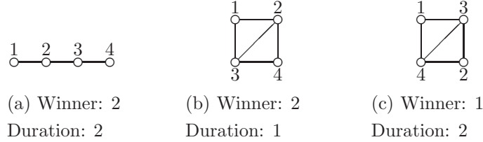
Figure 13: Examples with \delta_1 \leq (1/2)^{1/2} and \delta_{2,3,4} > (1/2)^{1/2}
