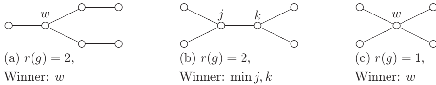
Figure 3: Pairwise stable networks for \delta \leq 1/2 .
